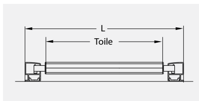
Guidage coulisses
